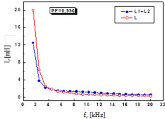
Figure 3. Inductance of L filter and LCL filter as function of switching frequency f_c , for PF = 0,996 .
