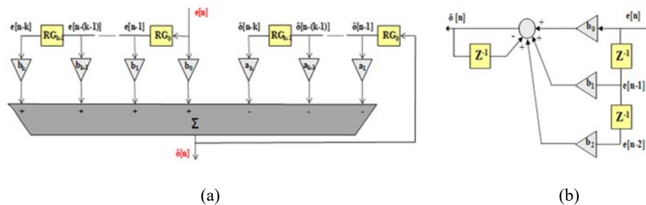
Figure.7. (a). Direct representation of differentials equation and (b). Operating modes Linear Regulator
