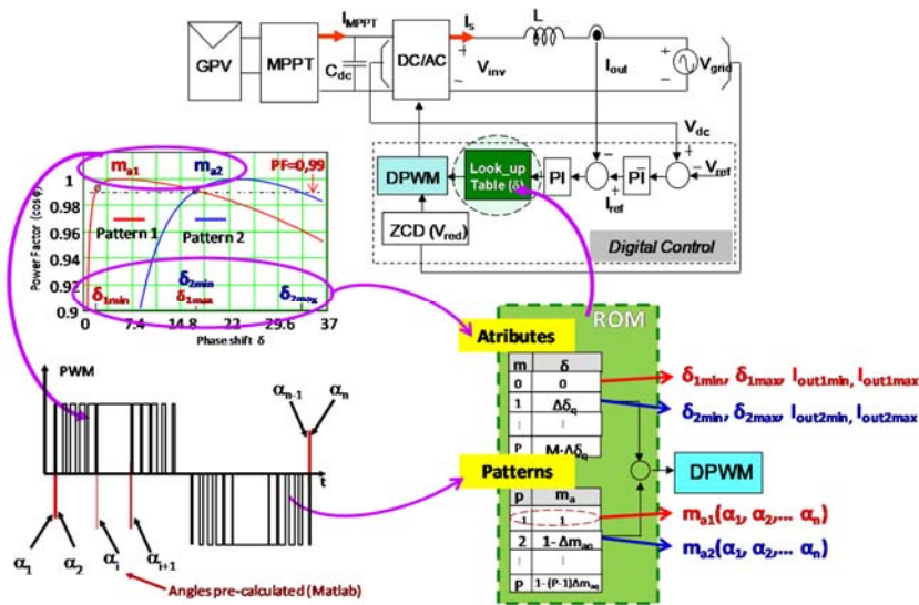
Figure 5. Scheme of the proposed control implementation
