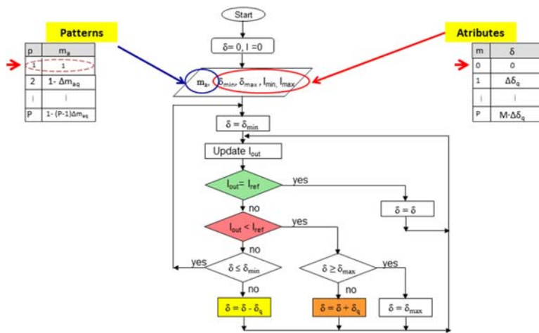
Figure 6. Control algorithm
